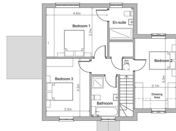
First Floor 1:100
