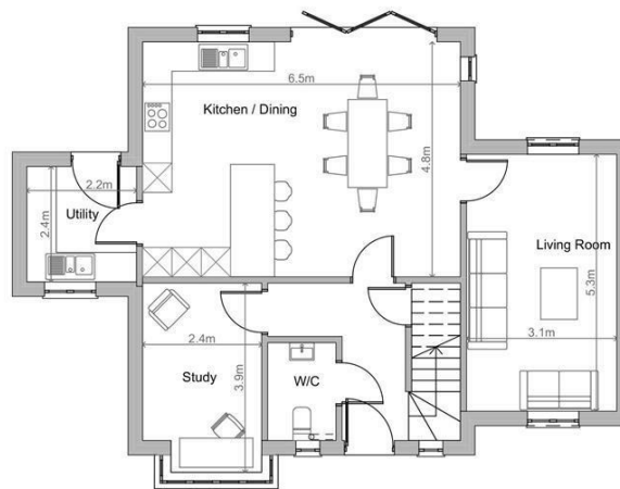
Ground Floor 1:100
